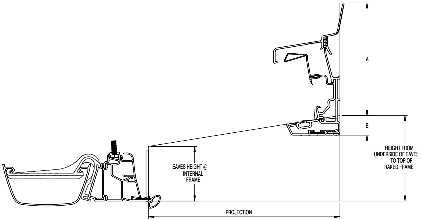
VENTILATED WALL PLATE HEIGHT RESTRICTION DETAILS
