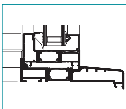
Cill/fix light
