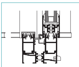
HSW sill
